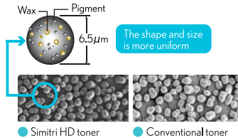
Comparison of conventional toner and Simitri HD toner. (Internal testing)
